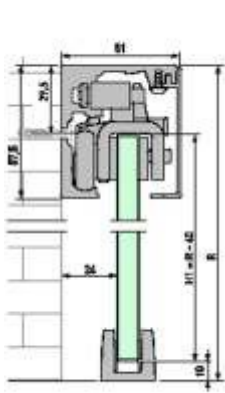
Detalle pared
