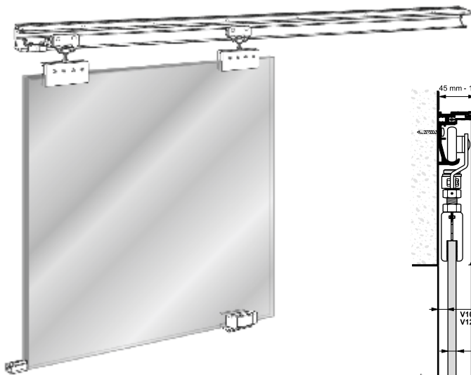
ALZADO KT GLAS 180 EXPERT
