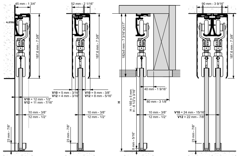
ALZADO KT GLAS 180 EXPERT
